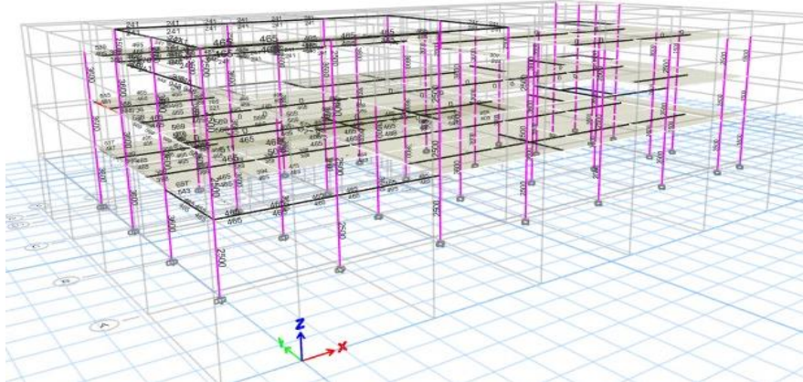
Gambar 2. Pengecekan Tulangan 3D
