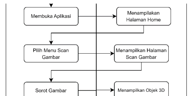
Gambar 4. Activity Diagram scan gambar
