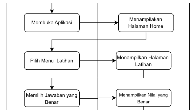
Gambar 5. Activity Diagram Latihan
