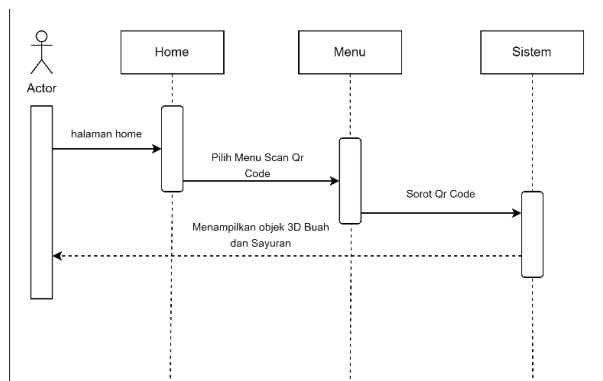
Gambar 6. Sequence Diagram Scan qr code
